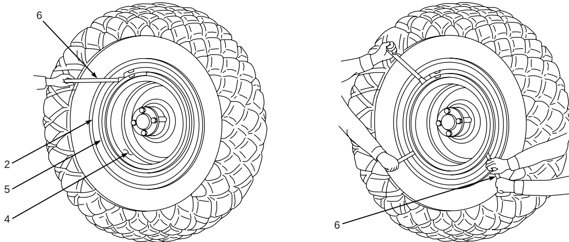
Figure 26. Installing Lockring
