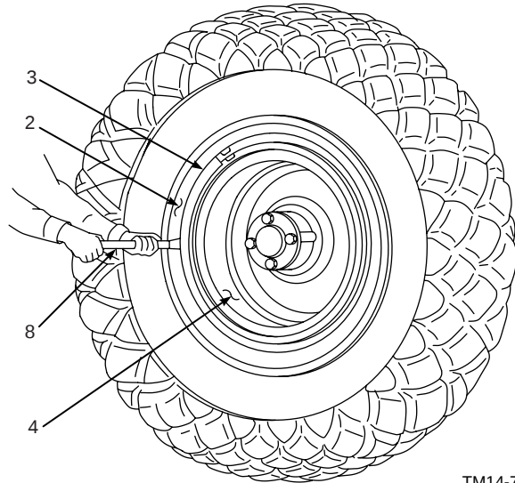
Figure 20. Removal of Outer Rim Flange
